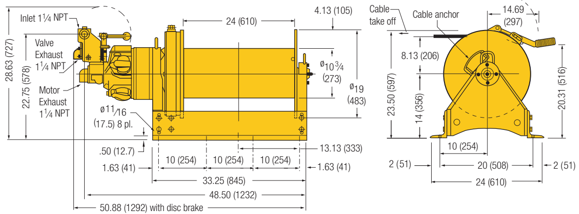
FA2.5MR24MK1G with disc and manual brake in inches (mm)
