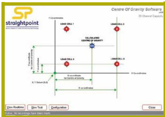
Home Screen
